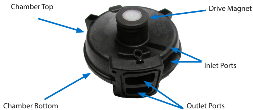
Completed Chamber Assembly
